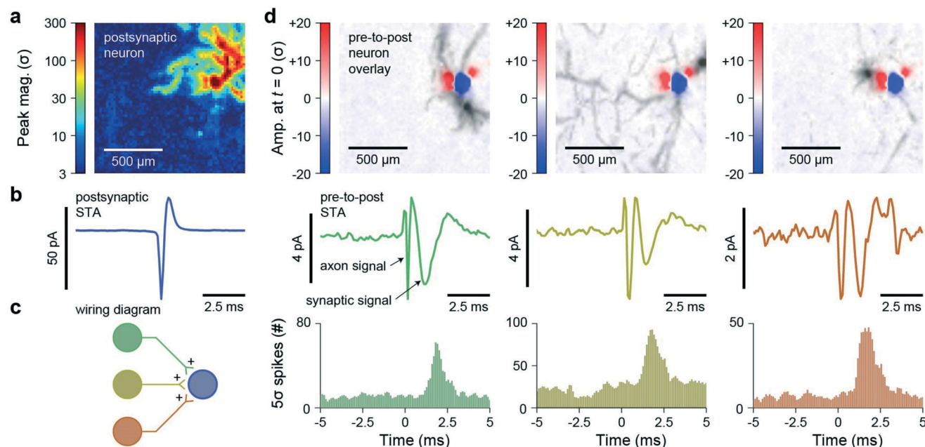
Fig. 3 Mapping synaptic connections using spike-triggered-averaging and cross-correlation. a–c, A post synaptic neuron, with its spike-triggered-average (STA) electrical imprint and soma STA shown in (b), has multiple excitatory synaptic inputs (c). d, Pre-to-post overlays show that the soma/AIS or dendrites of the post-synaptic neuron overlay axon branches from the respective pre-synaptic neurons allowing for synapse formation. The three pre-to-post STA signals each show a synaptic signal following the axon propagation signal which are time correlated with the pre-to-post cross correlograms confirming the direct synaptic connections.
